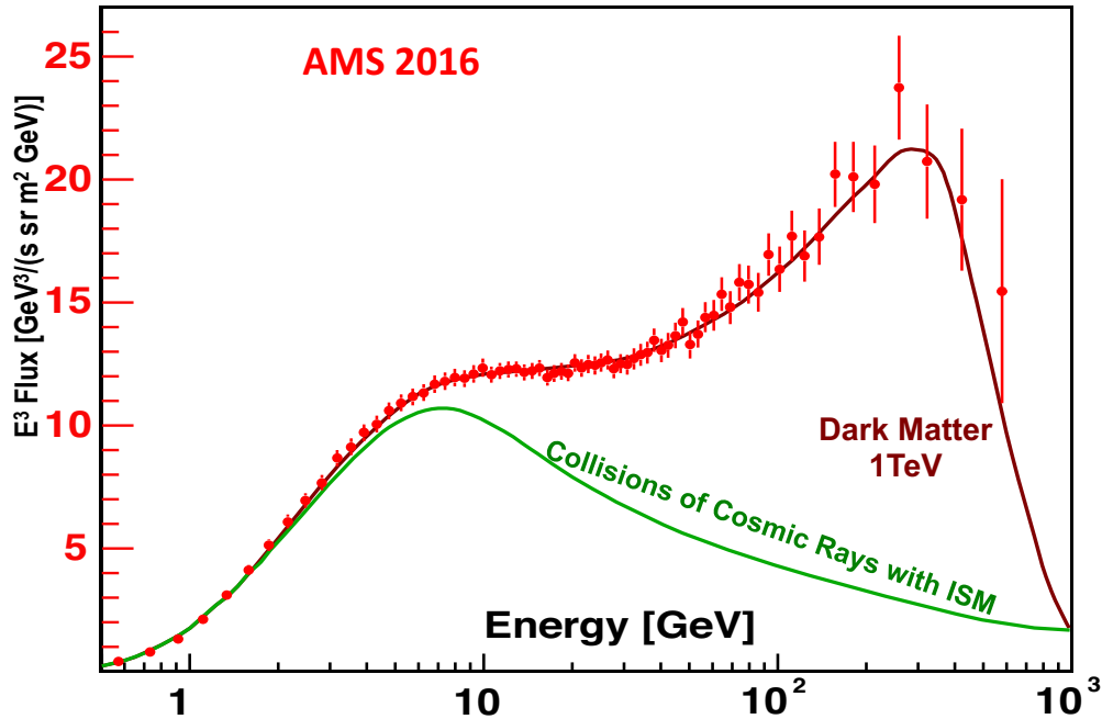
Figure 4. The current AMS positron flux measurement compared with theoretical models.
